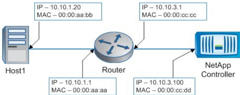
Figure 4-7) Traffic Flow
