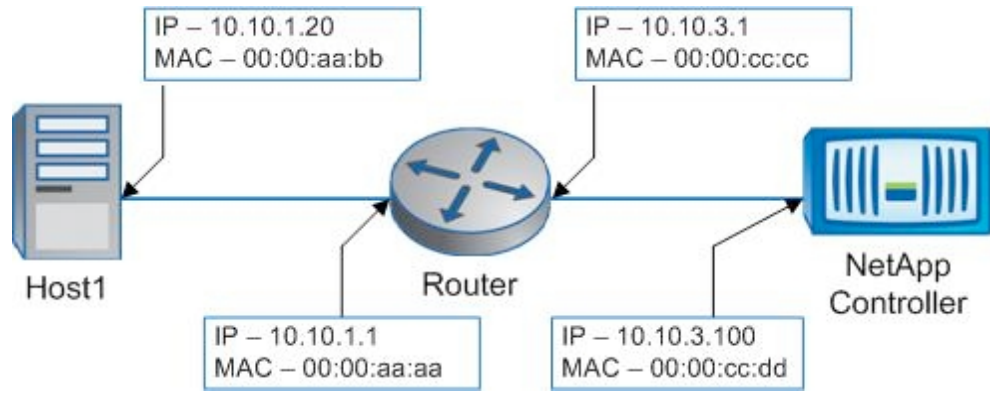
Figure 4-6 ) Traffic Flow
