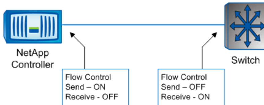
Figure 6-1) Flow Control
