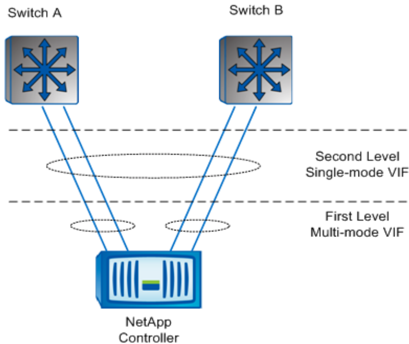
Figure 4-9) Layered VIF Example
