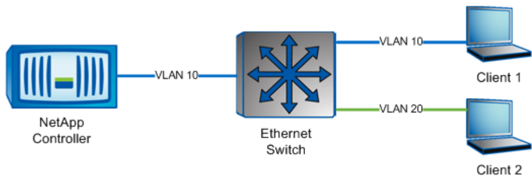
Figure 2-2) VLAN Description
