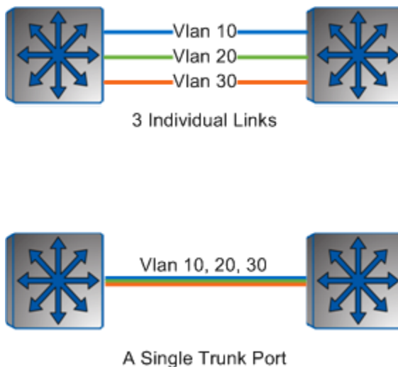
Figure 2-3 ) Vlan Trunking
