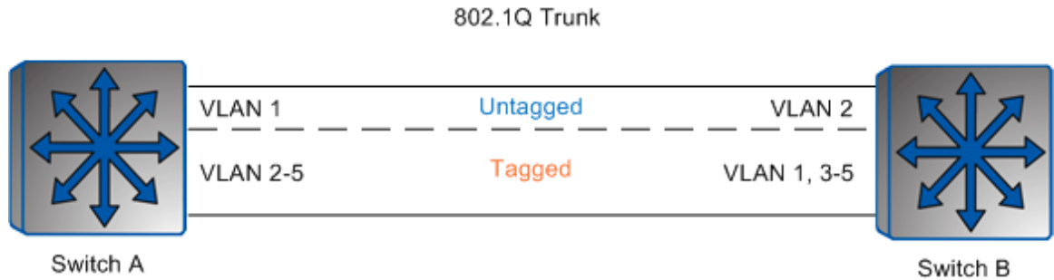
Figure 2-4) Native Vlan Misconfig
