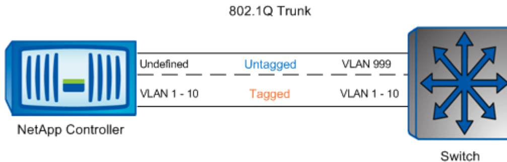
Figure 2-5 ) Native Vlan Netapp Config
