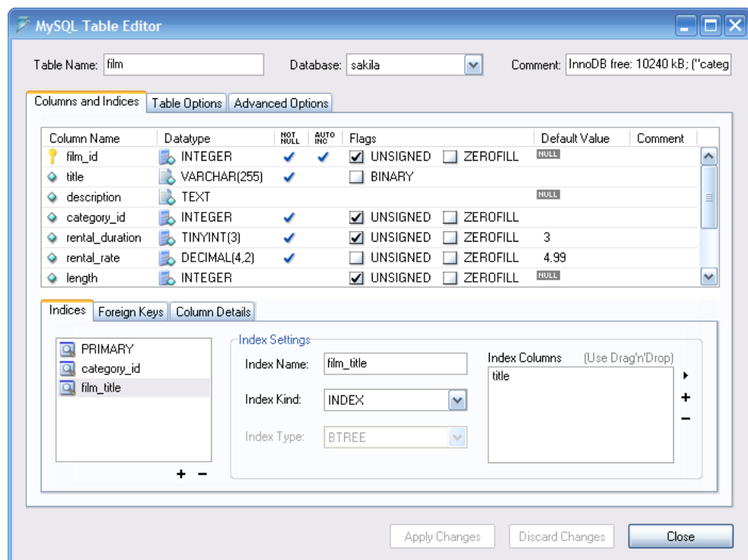
Figure 18.1. The MySQL Table Editor
