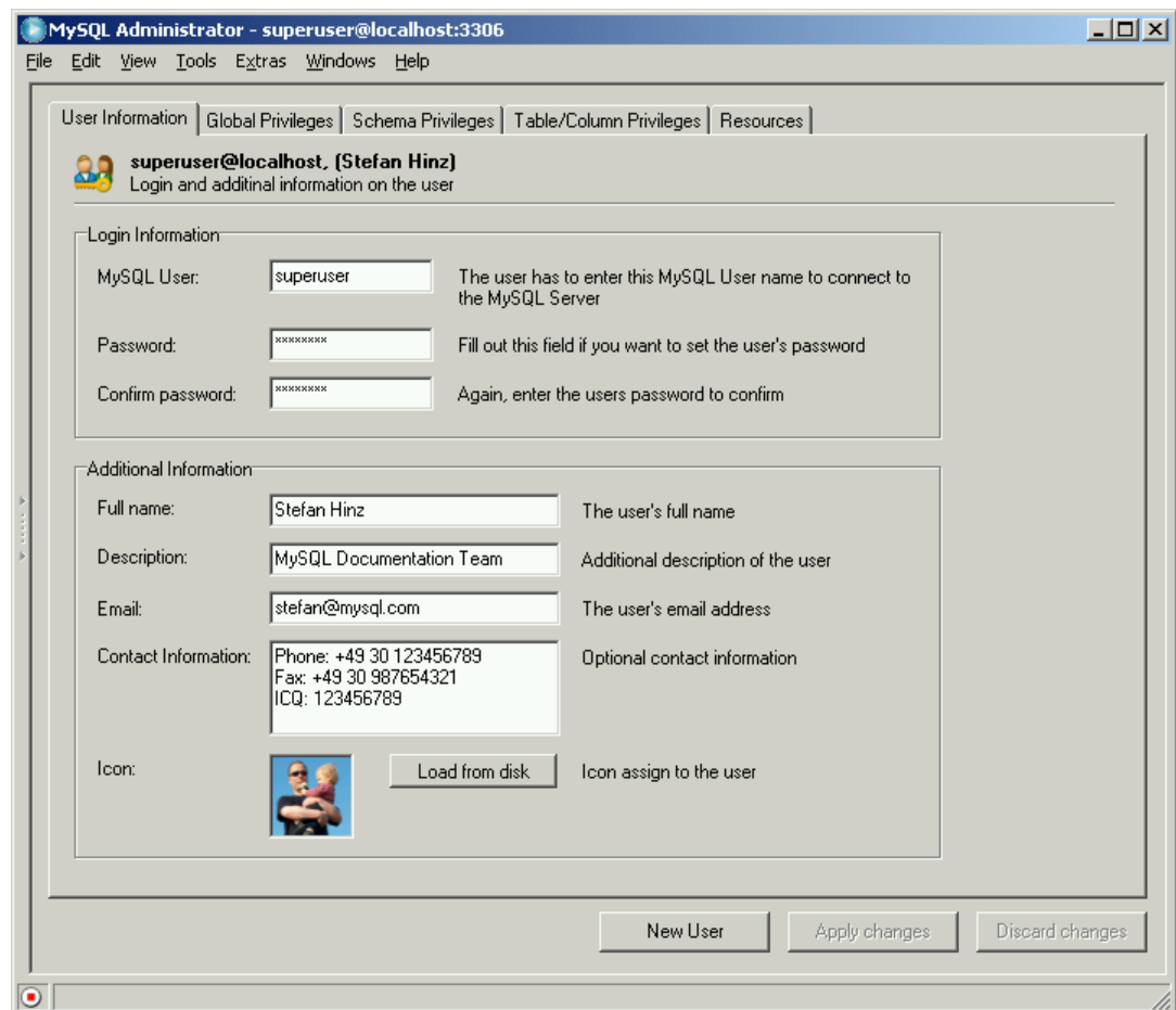
Figure 11.2. User Information tab
